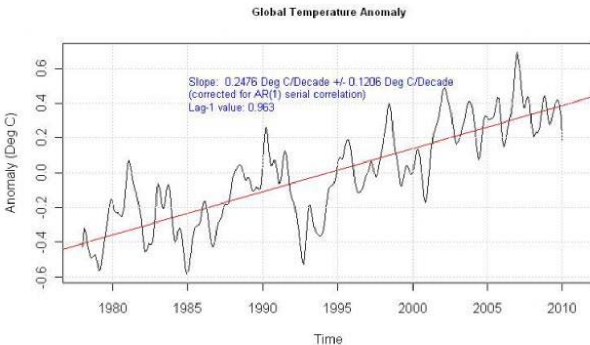
Figure 10 – Global temperatures as calculated from GHCN.
